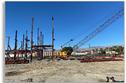
Steel Erection
